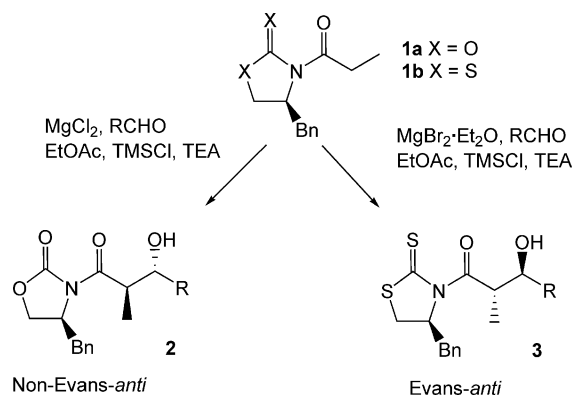
Scheme 1. Magnesium halide catalyzed anti -aldol reactions.
