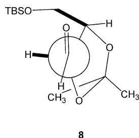
Figure 2. Newman projection of aldehyde 8.
