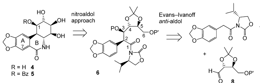
Scheme 2. Retrosynthetic analysis of 7-deoxypancratistatin 4.
