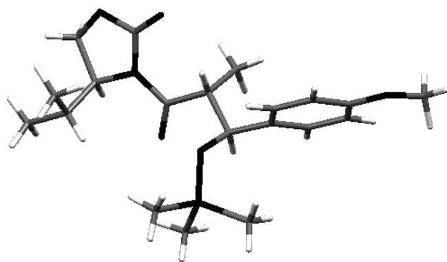
Figure 4. X-ray structure of 23 .
