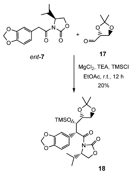
Scheme 5. anti -Aldol reaction of 2,3-acetonide-protected glyceraldehyde.
