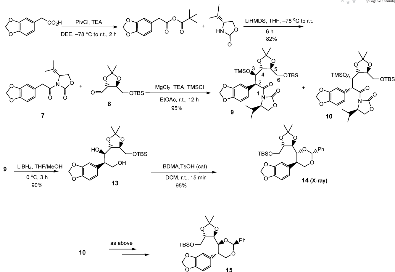
Scheme 3. Slight mismatched anti -aldol reaction.
