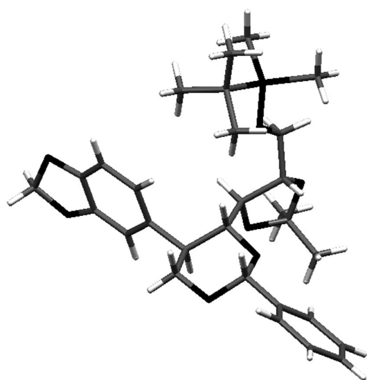
Figure 1. X-ray structure of 14 .
