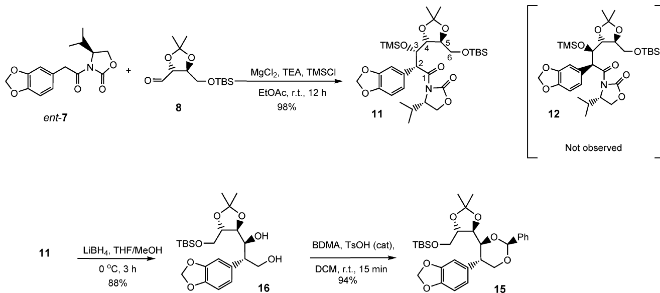
Scheme 4. Matched anti -aldol reaction.
