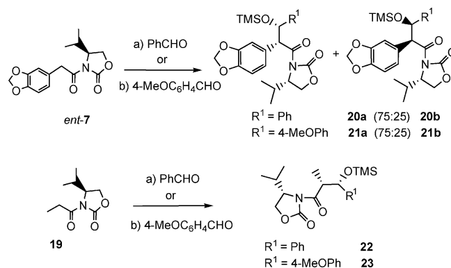
Scheme 6. anti -Aldol reactions with aromatic aldehydes.
