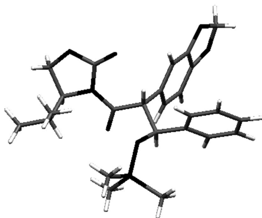
Figure 3. X-ray structure of 20a .
